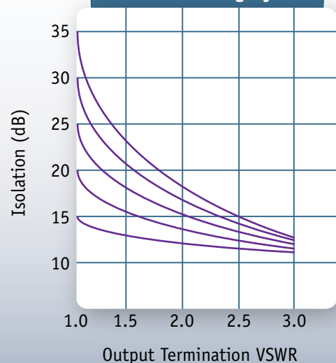
Isolation VS Output Termination VSWR For a Combining Hybrid
