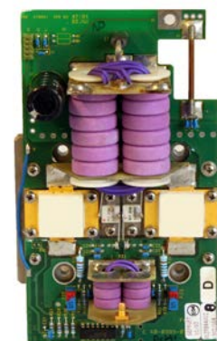
RF Amplifier Pallet
